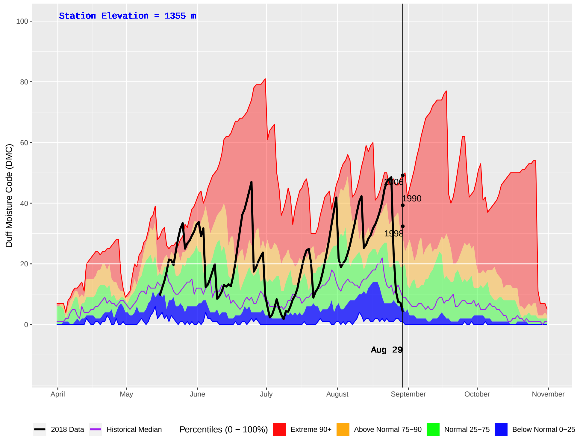
BIG VALLEY (262) : Historical (1987–2016) and Current (2018) Daily Duff Moisture Code (DMC)
