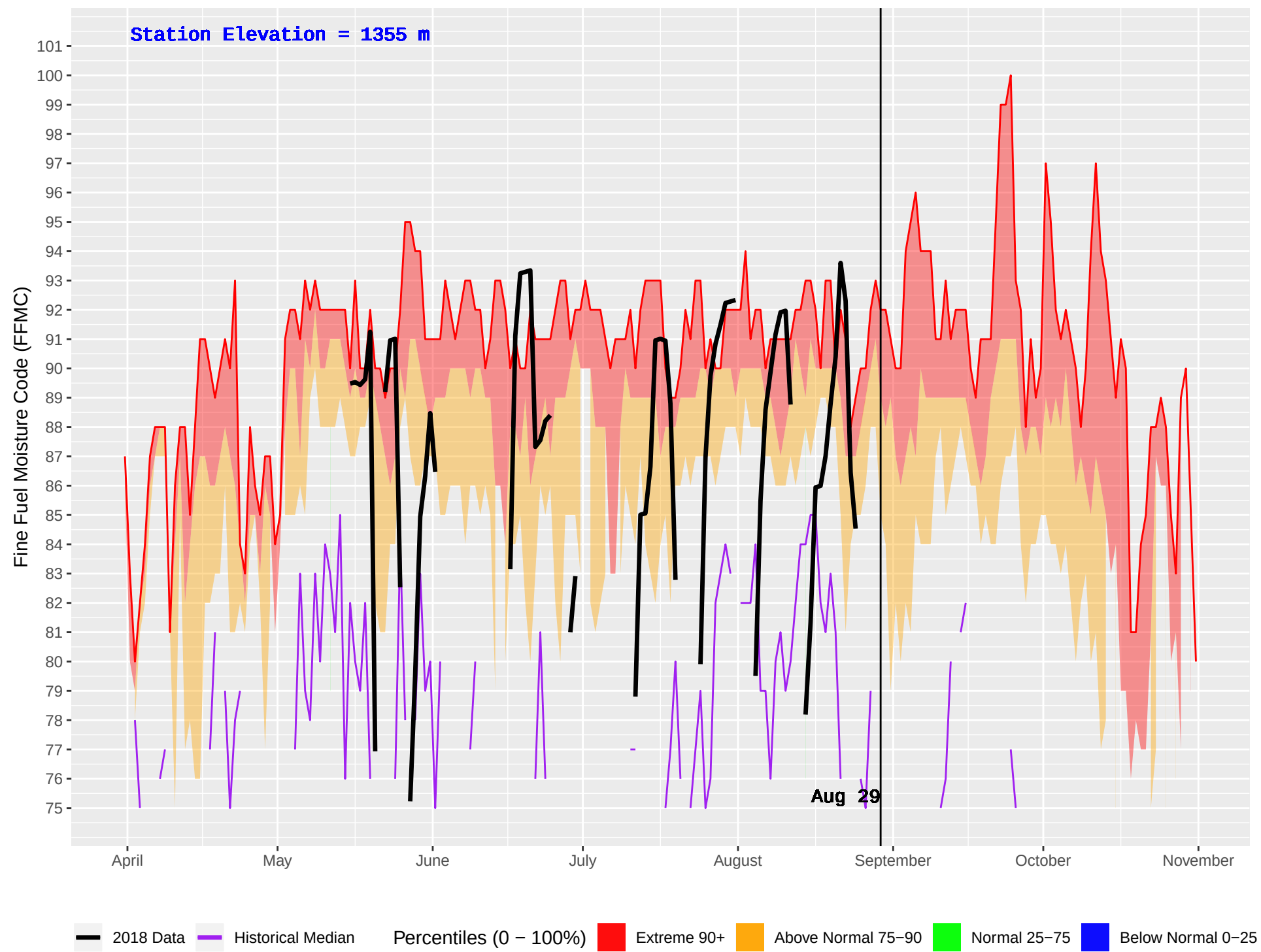
BIG VALLEY (262) : Historical (1987–2016) and Current (2018) Daily Fine Fuel Moisture Code (FFMC)
