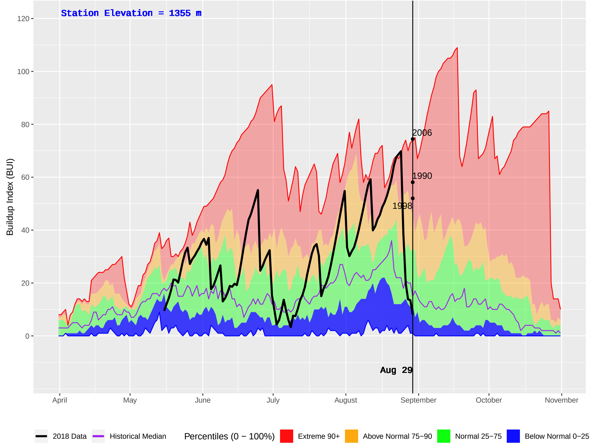
BIG VALLEY (262) : Historical (1987–2016) and Current (2018) Daily Buildup Index (BUI)
