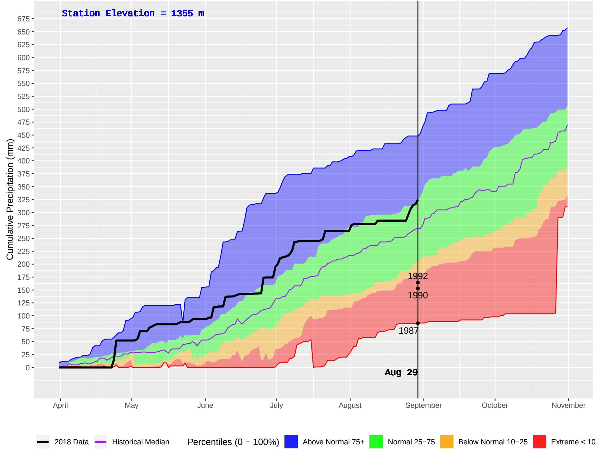
BIG VALLEY (262) : Historical (1987–2016) and Current (2018) Daily Cumulative Precipitation
