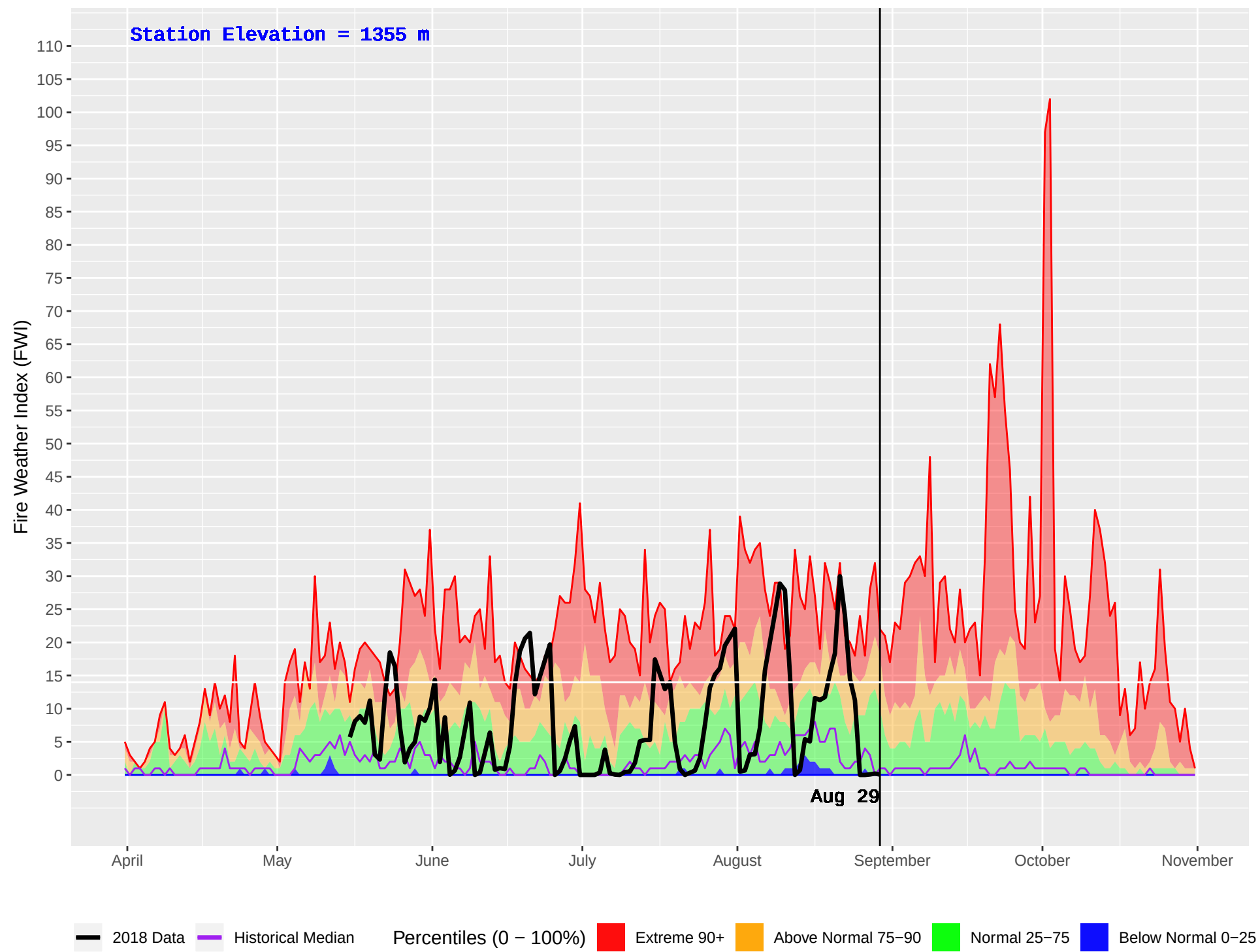
BIG VALLEY (262) : Historical (1987–2016) and Current (2018) Daily Fire Weather Index (FWI)
