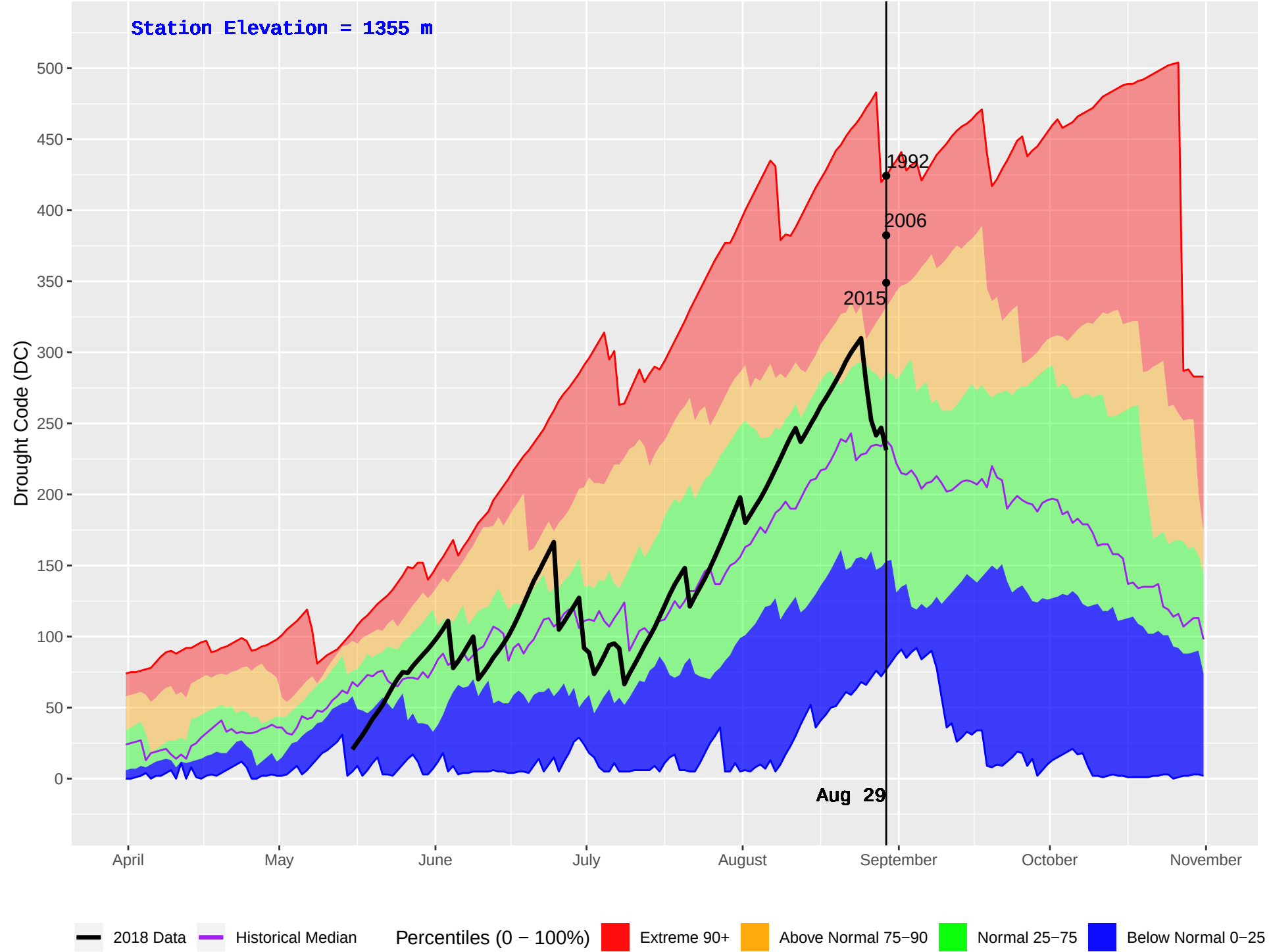
BIG VALLEY (262) : Historical (1987–2016) and Current (2018) Daily Drought Code (DC)
