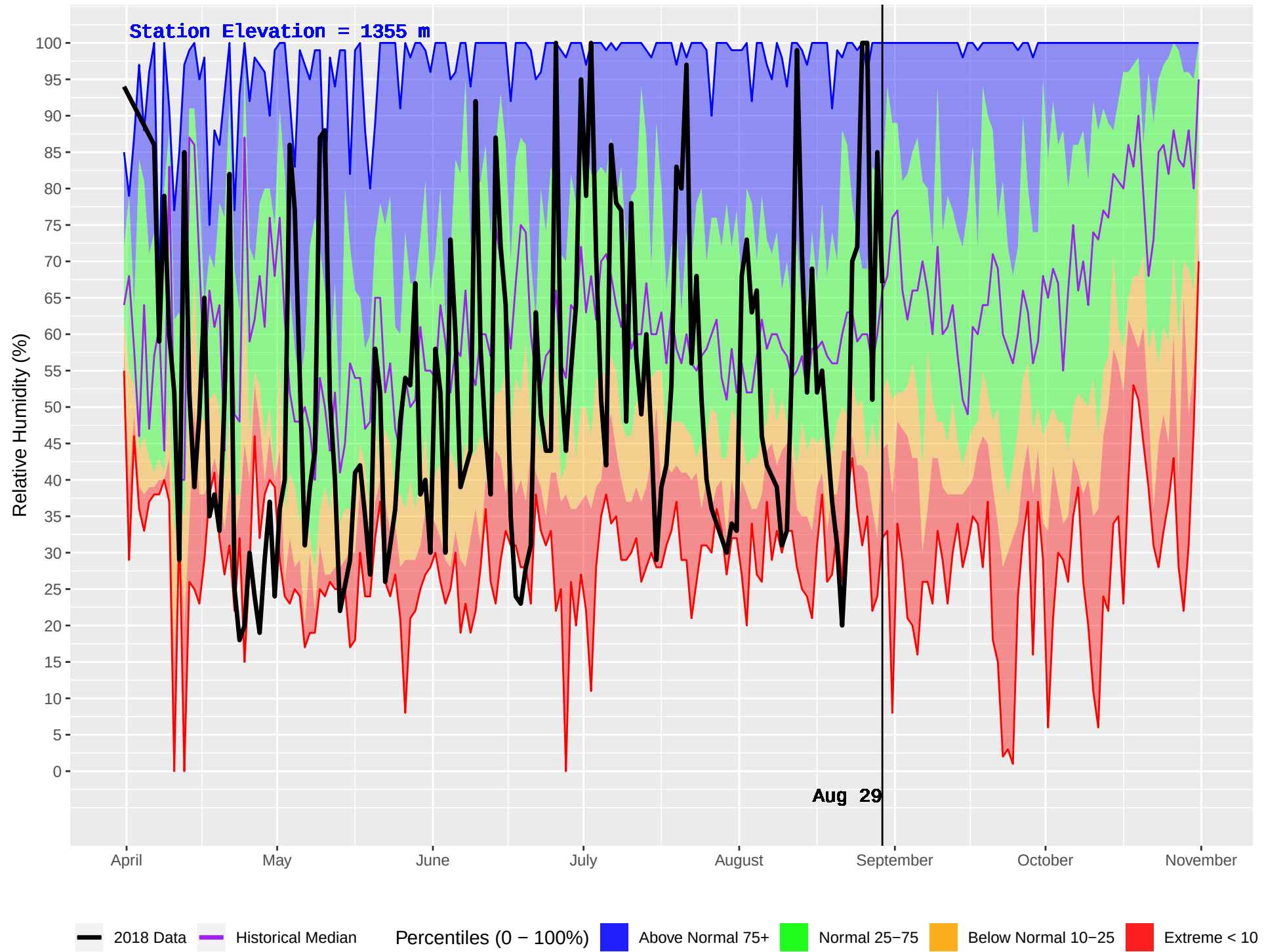
BIG VALLEY (262) : Historical (1987–2016) and Current (2018) Daily Relative Humidity
